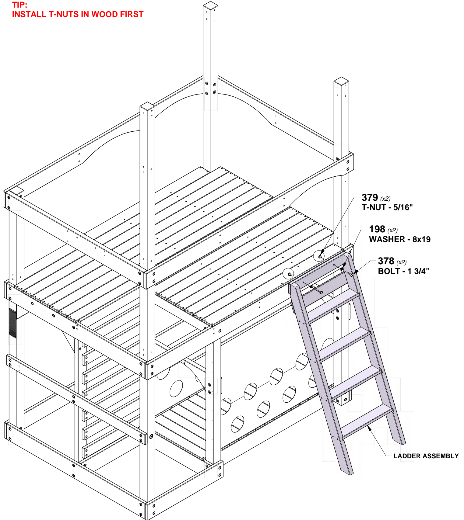
LADDER ASSEMBLY
